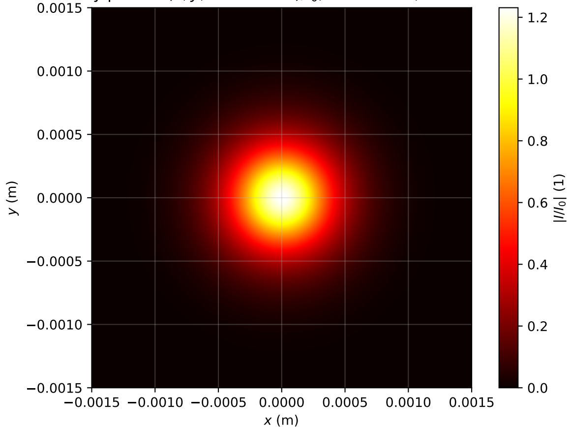
Intensity profile I(x, y, z = 0.796m)/I_0 , \text{Pin}=0.8\text{Pcr} , artificial time
